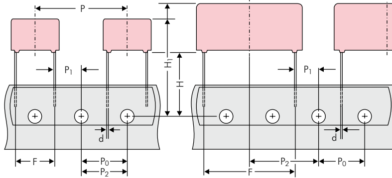
Diagram 2: PCM 10/15 mm
