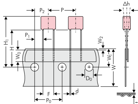
Diagram 1: PCM 2.5/5/7.5mm
