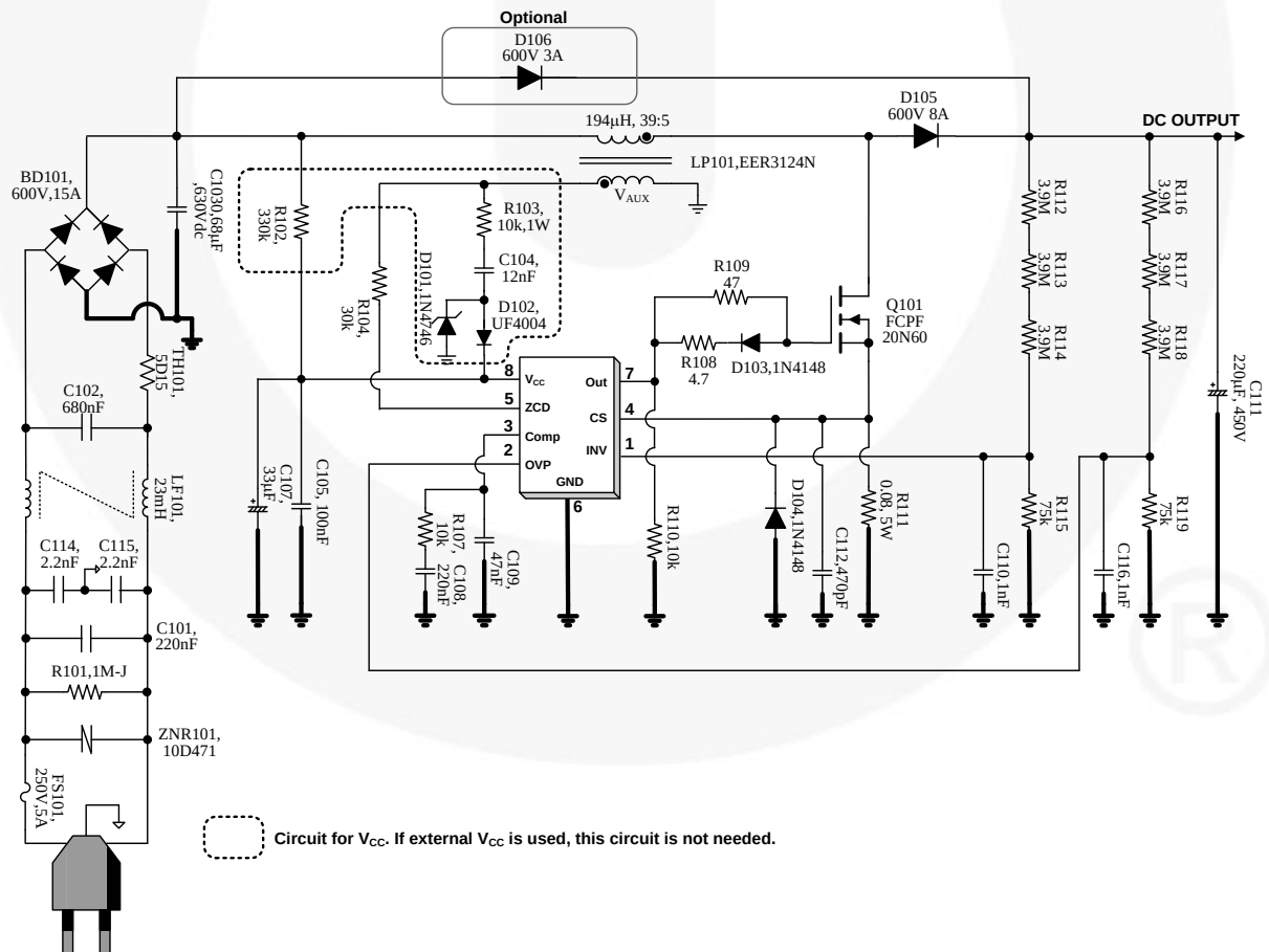
Figure 45. Demonstration Circuit
