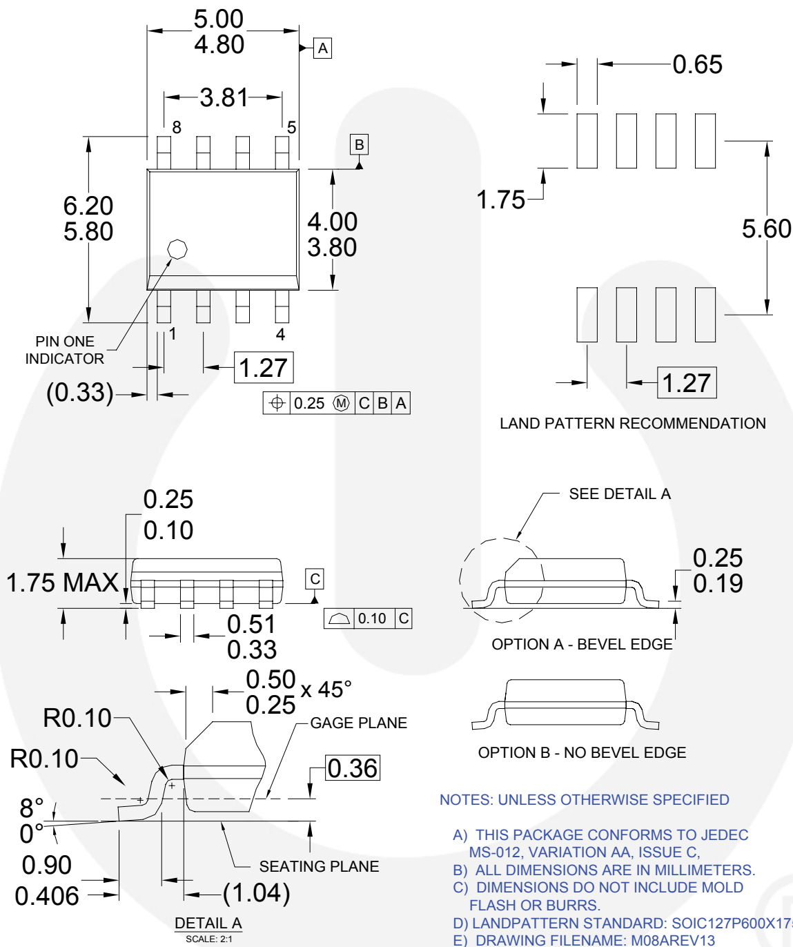
Figure 19. SOIC-8 Package
