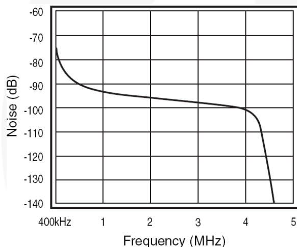
Figure 6. SD Noise vs. Frequency
