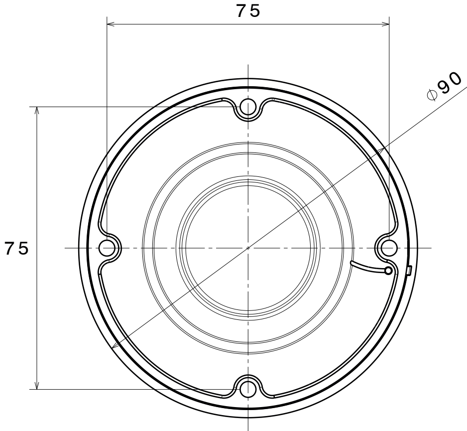
Bottom view
