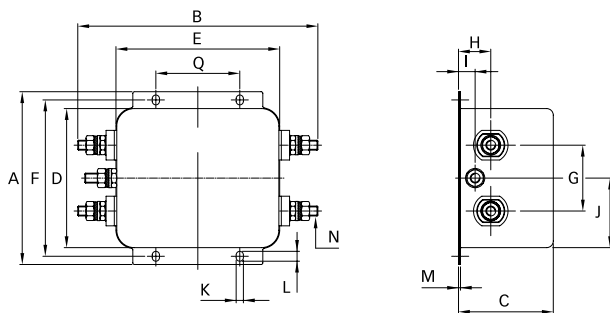
Connection style -24
