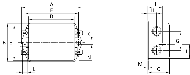
Connection style -06, 1 to 12 A types
