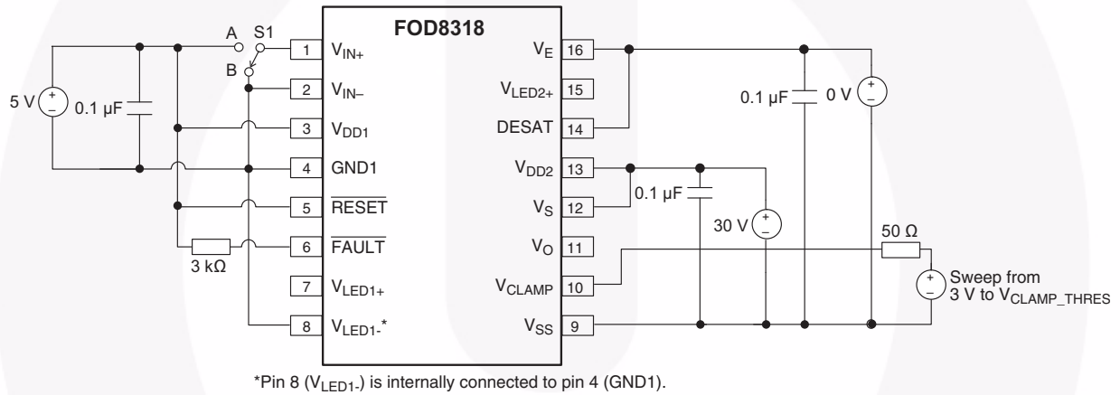
Figure 52. Clamp Pin Threshold Voltage ( V_{CLAMP} )
