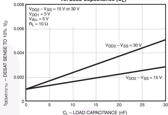
Figure 26. DESAT Sense to 10 % V_{\text{O}} Delay ( t_{\text{DESAT(10\%)}} ) vs. Load Capacitance ( C_{\text{L}} )
