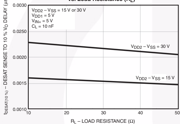
Figure 27. DESAT Sense to 10 % V_{\text{O}} Delay ( t_{\text{DESAT(10\%)}} ) vs. Load Resistance ( R_{\text{L}} )
