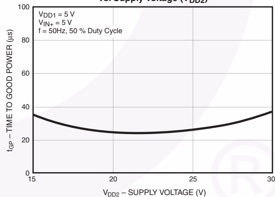
Figure 30. Time to Good Power ( t_{\text{GP}} ) vs. Supply Voltage ( V_{\text{DD2}} )
