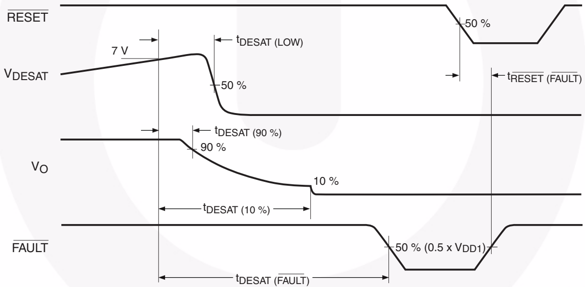
Figure 54. Definitions for Fault Reset Input ( \overline{\text{RESET}} ), Desaturation Voltage Input (DESAT), Output Voltage ( V_O ), and Fault Output (FAULT) Timing Waveforms
