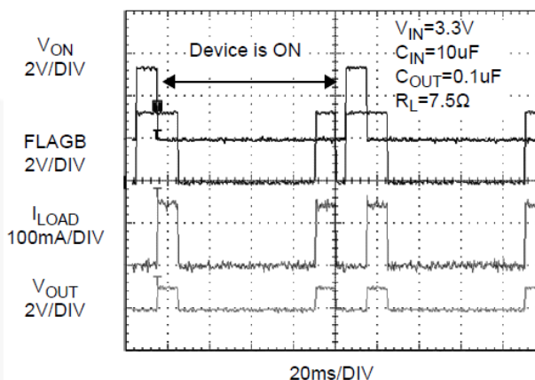
Figure 24. PPF2025 T_{BLANK} and T_{RESTART} (Active LO Device)
