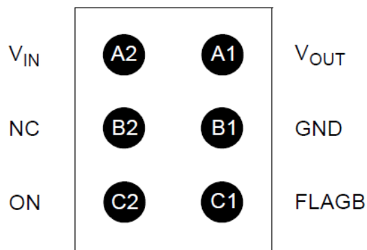
Figure 4. Pin Assignment 1.0 x 1.5 CSP Bottom View
