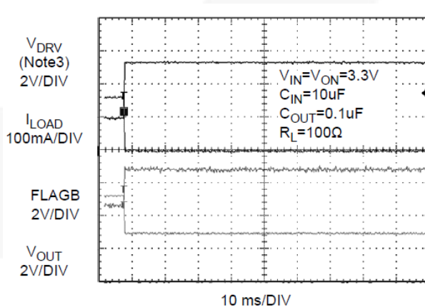
Figure 22. PFP2027 Over-Current (3) Over-Current condition is applied while device in normal operation (FLAGB inserts immediately and reports the fault condition)
