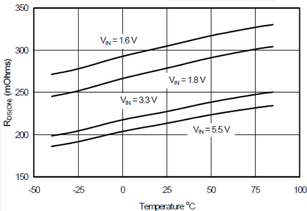
Figure 10. R_{DS(ON)} vs. Temperature
