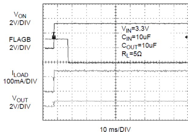
Figure 23. PPF2027 Startup FLAGB Blanking Time
