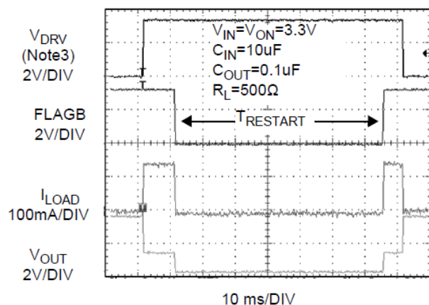
Figure 17. PFP2024 T_{RESTART} Response (3)
