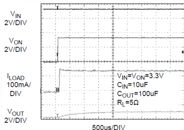
Figure 19. PFP2024 Current Limit Response Time (Output is loaded by 5 \Omega and C_{OUT} = 100 \mu F )
