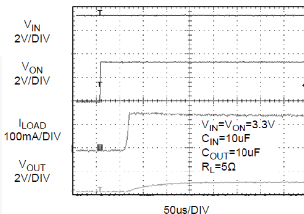
Figure 18. PFP2024 Current Limit Response Time (Output is loaded by 5 \Omega and C_{OUT} = 10 \mu F )
