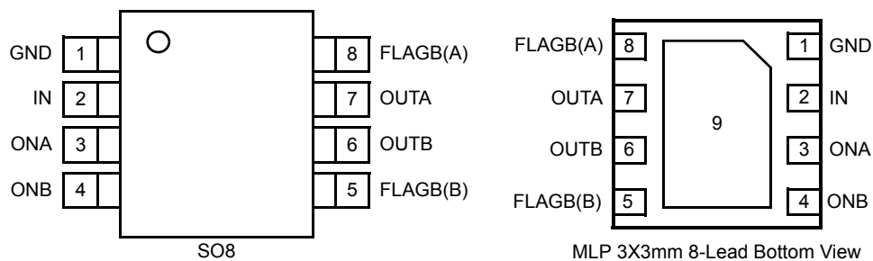
Figure 5. Pin Configurations
