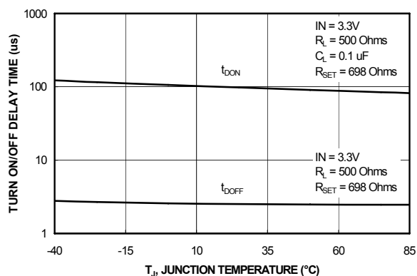
Figure 18. t_{ON} / t_{OFF} vs. Temperature
