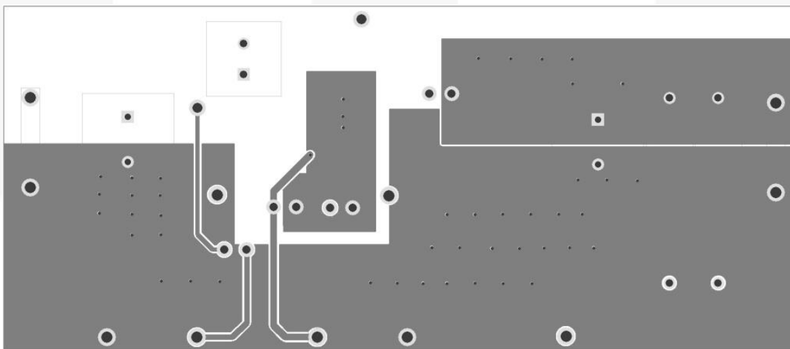
Figure 45. Bottom and ASB Layers
