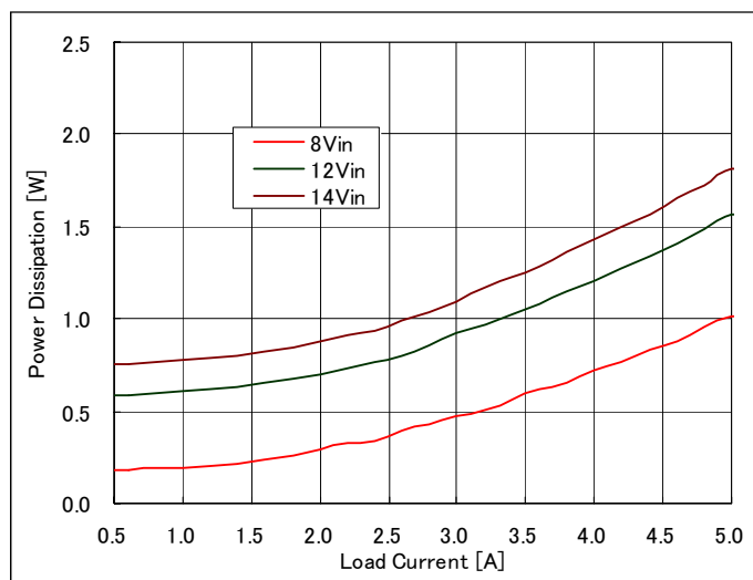
Fig 5.0V-3: Power Loss vs. load current and input voltage for V_{out}=5.0V . Airflow rate = 200LFM (1m/s) and T_a=25^{\circ}C .
