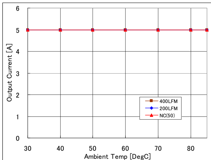
Fig 5.0V-1: Available load current vs. ambient temperature and airflow rates for V_{out}=5.0V with V_{in}=12V . Maximum component temperature \leq 120^{\circ}C .
