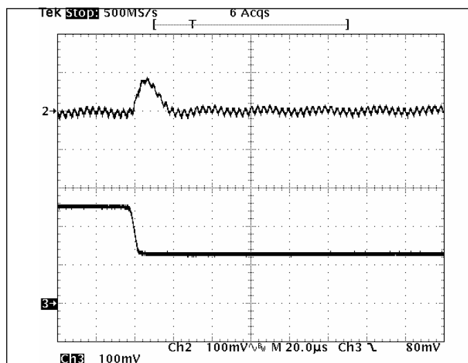
Fig 1.8V-7: Output voltage response for V_{out}=1.8V to negative load current step change from 5A to 2.5A with slew rate of -5A/\mu s at V_{in}=12V . C_o=47\mu F \times 2 ceramic. Top trace: output voltage (100mV/div.) Bottom trace: load current (2A/div.) Time scale: 20\mu s /div.
