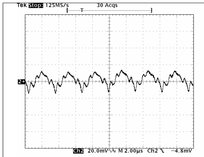
Fig 1.8V-5: Output voltage ripple (20mV/div.) for V_{out}=1.8V at full rated load current into a resistive load with external capacitance 47\mu F \times 2 ceramic + 1\mu F ceramic at V_{in}=12V . Time scale: 2\mu s /div.
