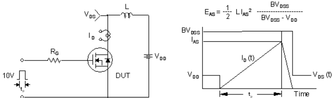
Unclamped Inductive Switching Test Circuit &amp; Waveforms
