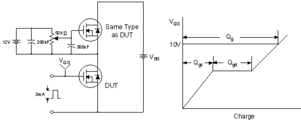
Resistive Switching Test Circuit &amp; Waveforms
