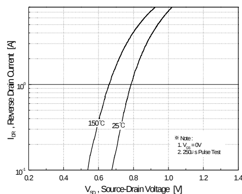
Figure 4. Body Diode Forward Voltage Variation vs. Source Current and
