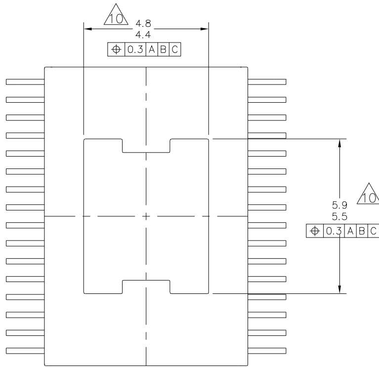
VIEW C-C
