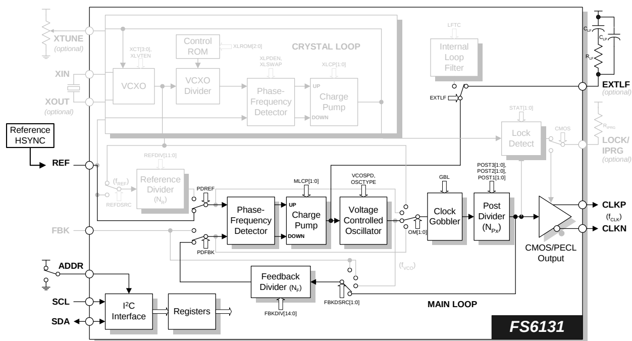
Figure 25: Block Diagram: Line-Locked Clock Generation
