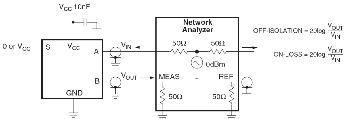
Figure 9. Off Isolation
