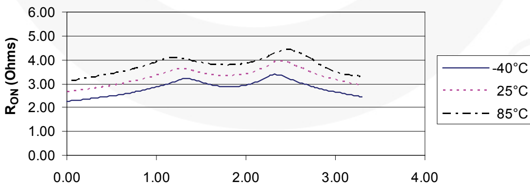
Figure 6. R_{ONVID} , V_{IN} , V_{AV} = 3.0V , V_{BUS} = 0V
