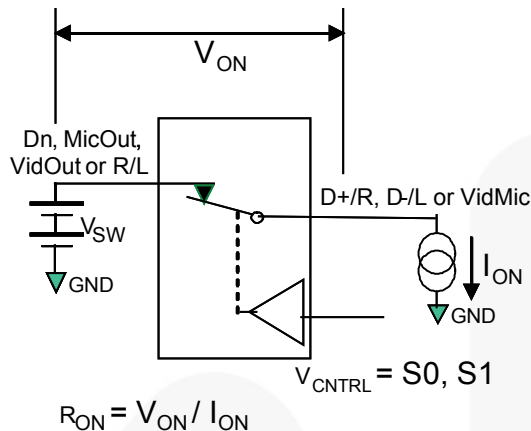
Figure 14. On Resistance
