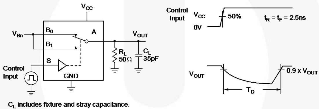
Figure 12. Break-Before-Make Timing
