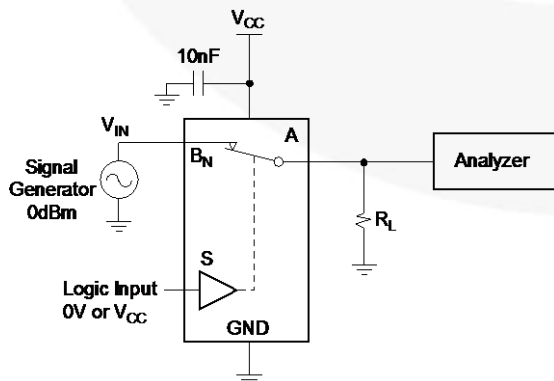
Figure 16. Bandwidth
