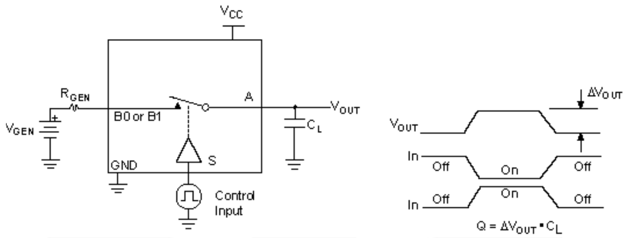
Figure 14. Charge Injection
