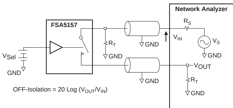
Figure 6. OFF Isolation
