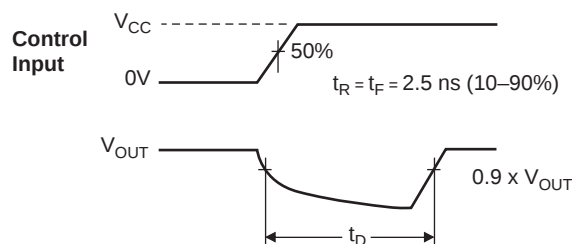
Figure 5. Break-Before-Make Timing
