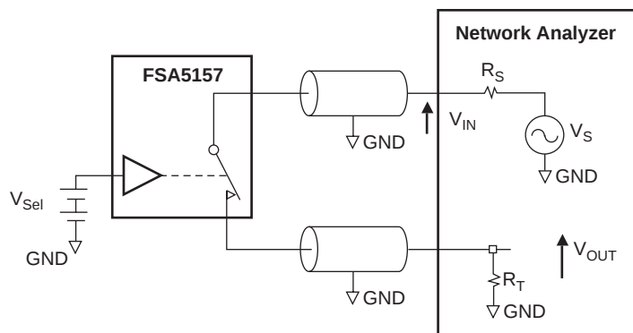
Figure 10. Bandwidth
