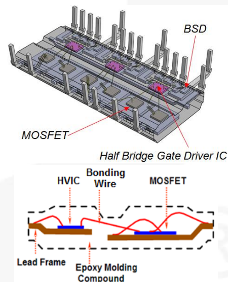
Figure 4. Package Structure
