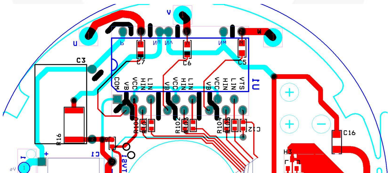
Figure 36. PCB Layout Example
