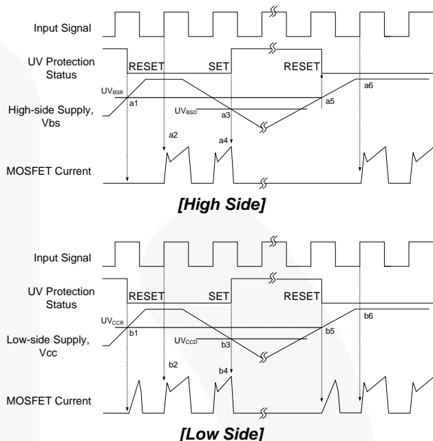
Figure 15. Timing Chart of Under-Voltage Protection
