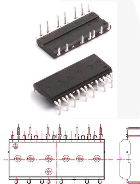
Figure 8. Zigzag DIP Package
