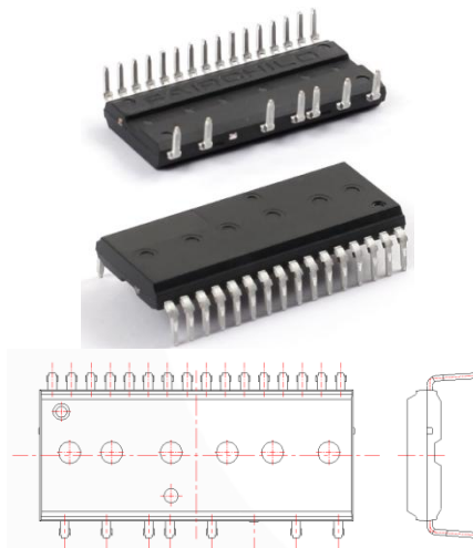
Figure 5. DIP Package
