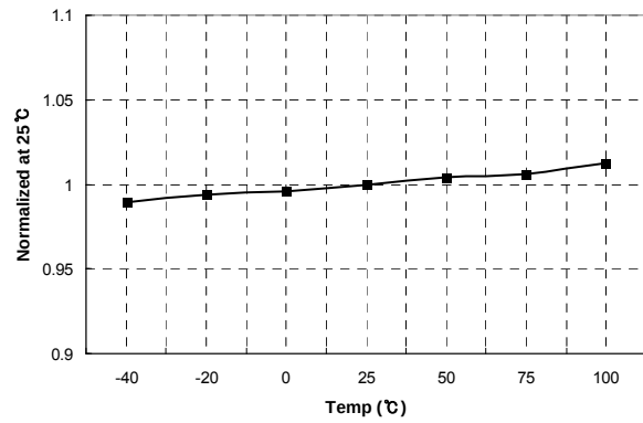
Figure 16. V LIM Voltage vs. Temperature
