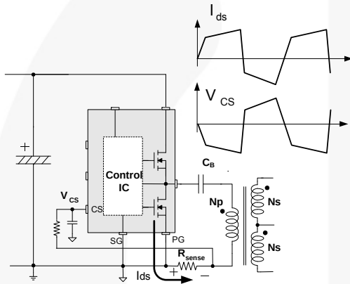
Figure 22. Full-Wave Sensing
