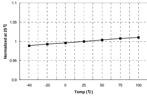
Figure 14. R T Voltage vs. Temperature
