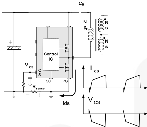
Figure 21. Half-Wave Sensing
