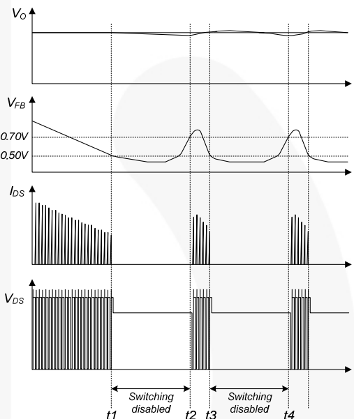
Figure 23. Burst-Mode Operation
