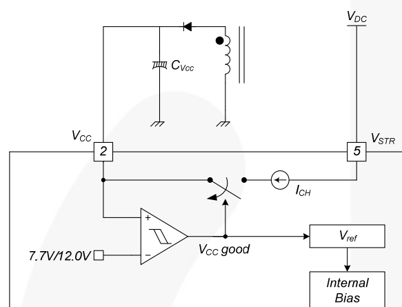
Figure 17. Startup Block
