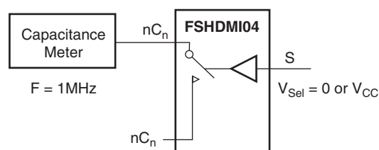
Figure 12. Channel ON-Capacitance
