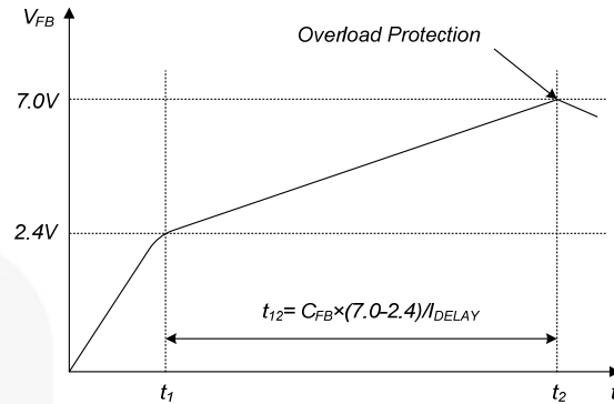
Figure 20. Overload Protection
