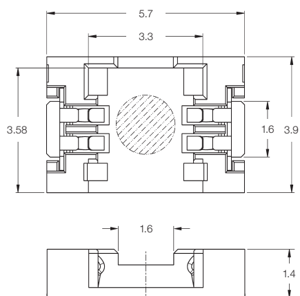
Board Connector
