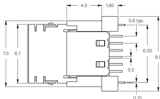
Plug
