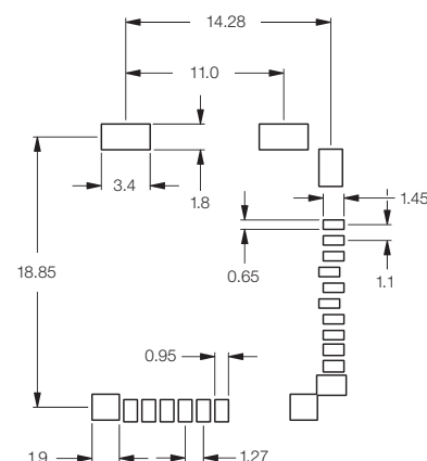
PCB Layout
