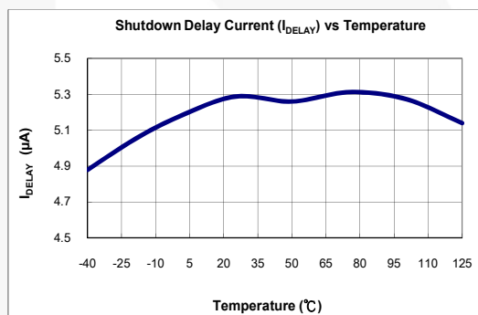
Figure 13. Shutdown Delay Current ( I_{DELAY} ) vs. Temperature
