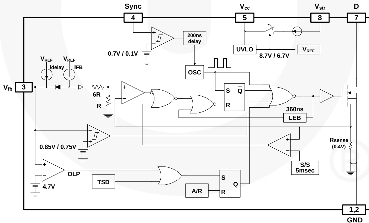
Internal Block Diagram
