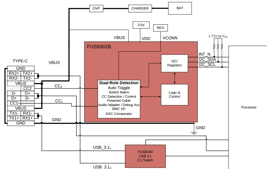
Figure 2. Typical Application
