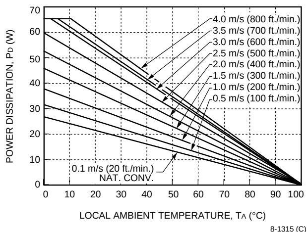
Figure 23. Convection Power Derating with No Heat Sink; Airflow Along Width (Transverse)
