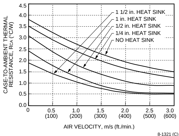
Figure 25. Case-to-Ambient Thermal Resistance Curves; Transverse Orientation
