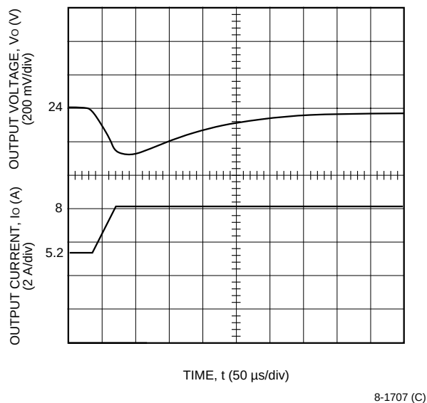
Figure 10. Typical FW250H1 Transient Response to Step Increase in Load from 50% to 75% of Full Load at Room Temperature and 48 V Input (Waveform Averaged to Eliminate Ripple Component.)
