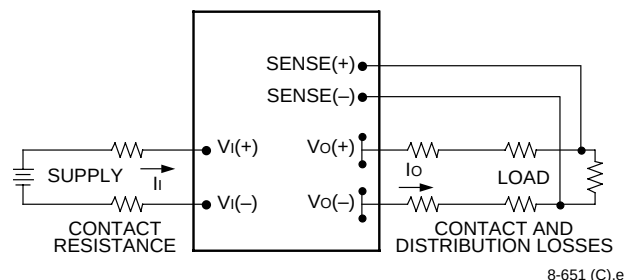
Figure 16. Effective Circuit Configuration for Single-Module Remote-Sense Operation
