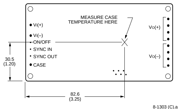
Figure 22. Case Temperature Measurement Location
