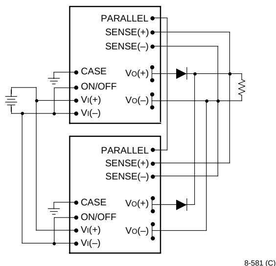
Figure 21. Wiring Configuration for Redundant Parallel Operation
