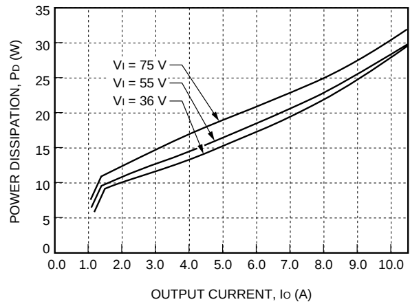
Figure 27. FW250H1 Power Dissipation vs. Output Current
