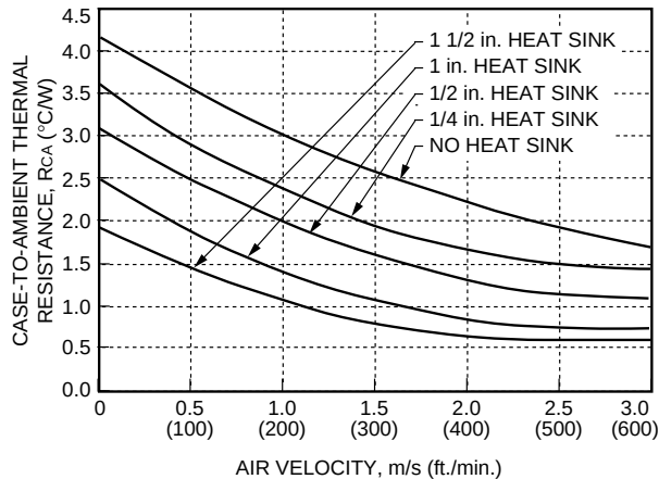
Figure 26. Case-to-Ambient Thermal Resistance Curves; Longitudinal Orientation
