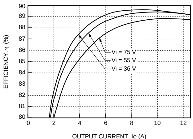
Figure 6. Typical FW300H1 Efficiency vs. Output Current at Room Temperature
