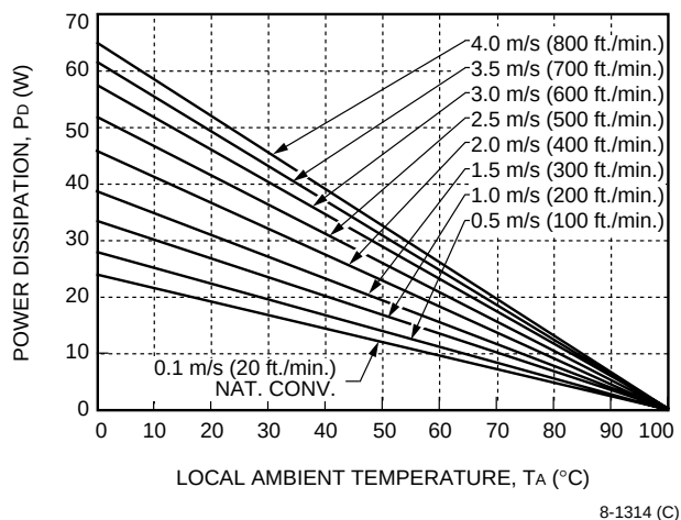
Figure 24. Convection Power Derating with No Heat Sink; Airflow Along Length (Longitudinal)
