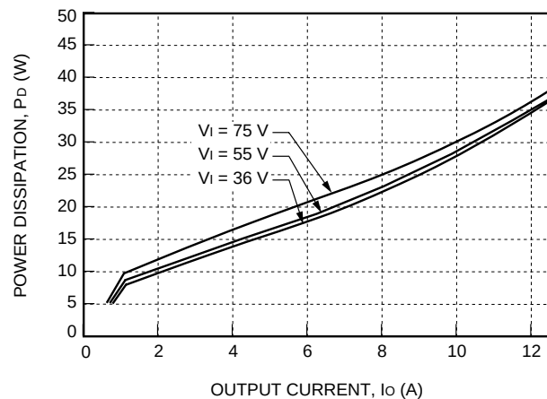
Figure 28. FW300H1 Power Dissipation vs. Output Current
