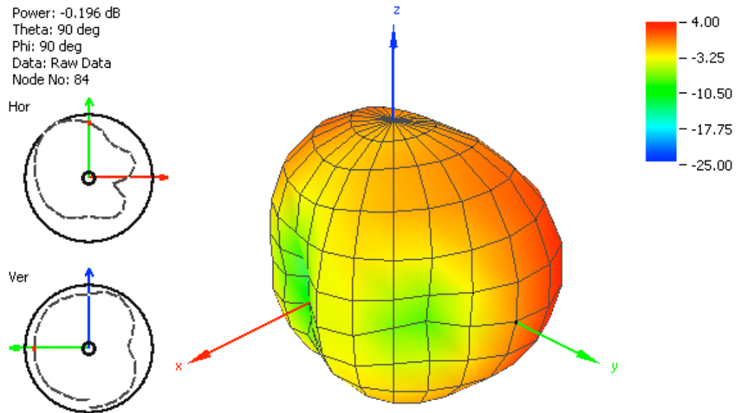
Figure 13. Radiation Pattern at 1850 MHz of FXUB66 UWB Antenna.
