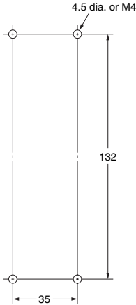
Panel Cutouts
