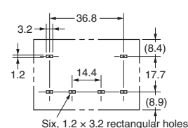
PCB Mounting Holes
