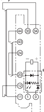
G7SA-3A1B Mounted
