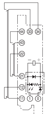
G7SA-2A2B Mounted
