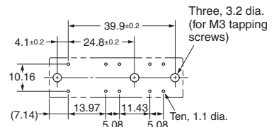
Mounting Hole Placement (Bottom View) (±0.1 tolerance)
