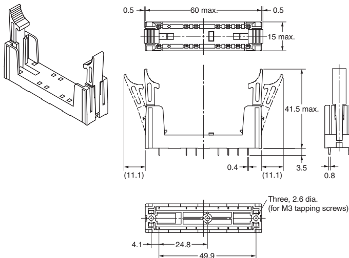
Terminal Arrangement/Internal Connection Diagram (Bottom View)
