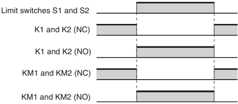
Timing Chart
