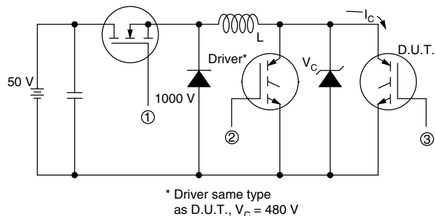
Fig. 14a - Switching Loss Test Circuit
