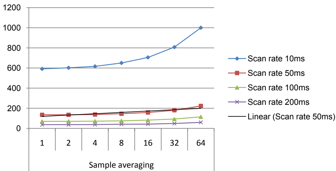
Figure 37-10. Power Consumption [ \mu A] 10 sensors, noise countermeasures Enabled, f=48\text{MHz} , V_{cc}=3.3\text{V}
