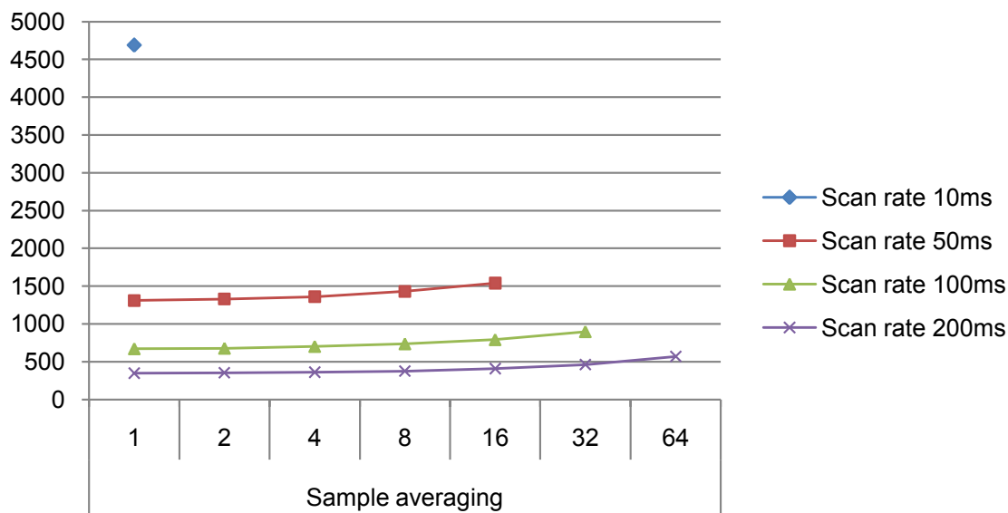
Figure 37-12. Power Consumption [ \mu A] 100 sensors, noise countermeasures Enabled, f=48\text{MHz} , V_{cc}=3.3\text{V}
