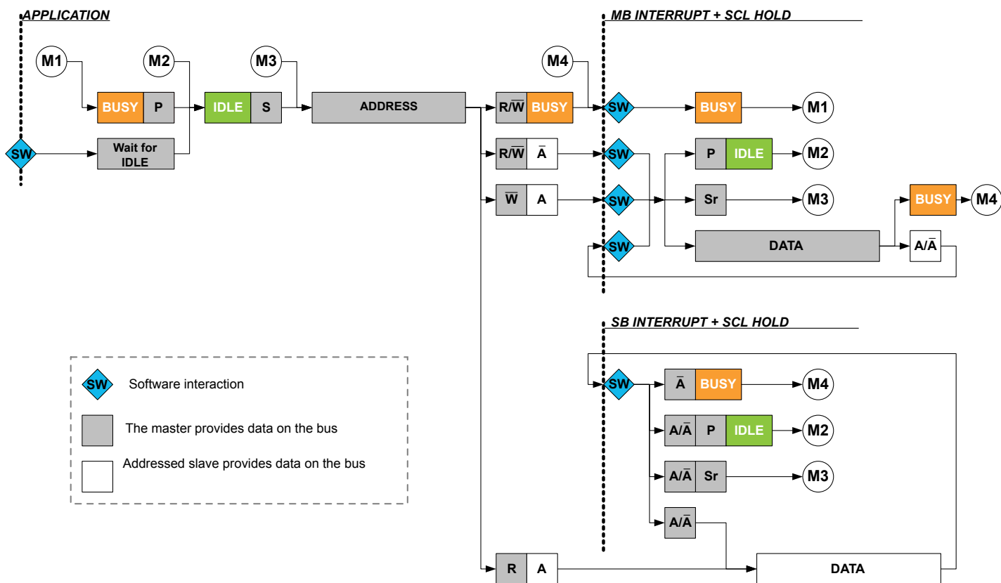
Figure 28-4. I 2 C Master Behavioral Diagram (SCLSM=0)
