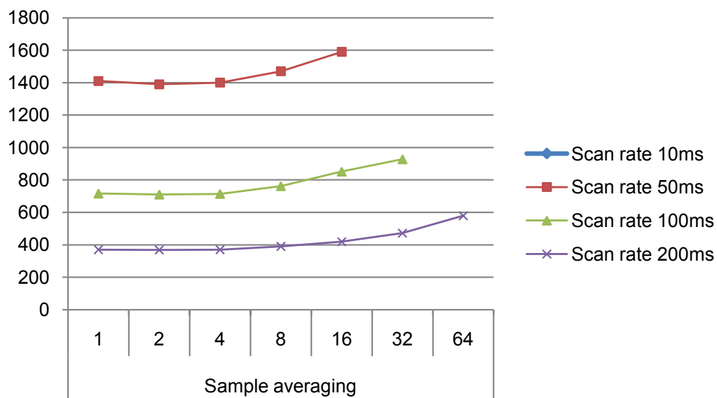
Figure 37-12. Power Consumption [ \mu A] 100 sensors, noise countermeasures Enabled, f=48\text{MHz} , V_{cc}=3.3\text{V}
