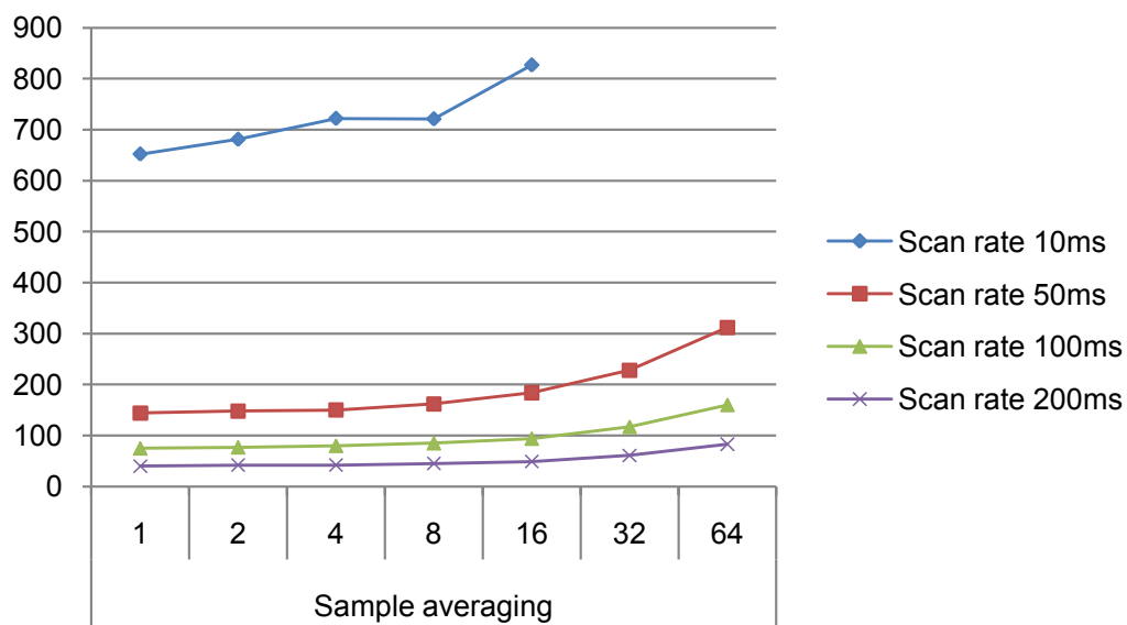
Figure 37-10. Power Consumption [ \mu A] 10 sensors, noise countermeasures Enabled, f=48\text{MHz} , V_{cc}=3.3\text{V}
