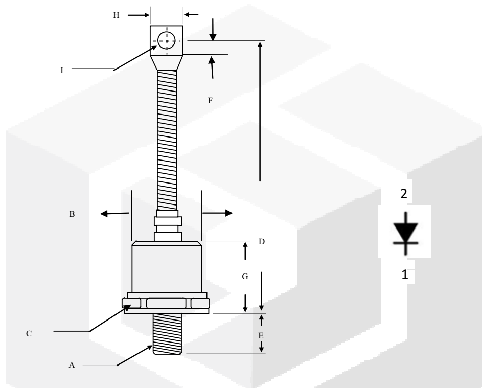
DO-9 (DO-205AB)
