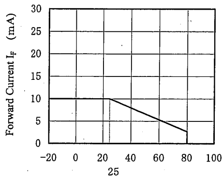
Case Temperature T_c (°C) Forward Current Derating Curve
