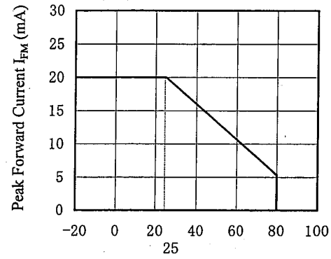
Case Temperature T_c (°C) Peak Forward Current Derating Curve
