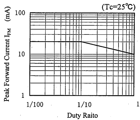
( T_c = 25^\circ\text{C} ) Duty Ratio Peak Forward Current vs. Duty Ratio
