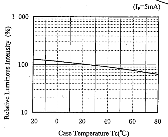
Relative Luminous Intensity vs. Case Temperature
