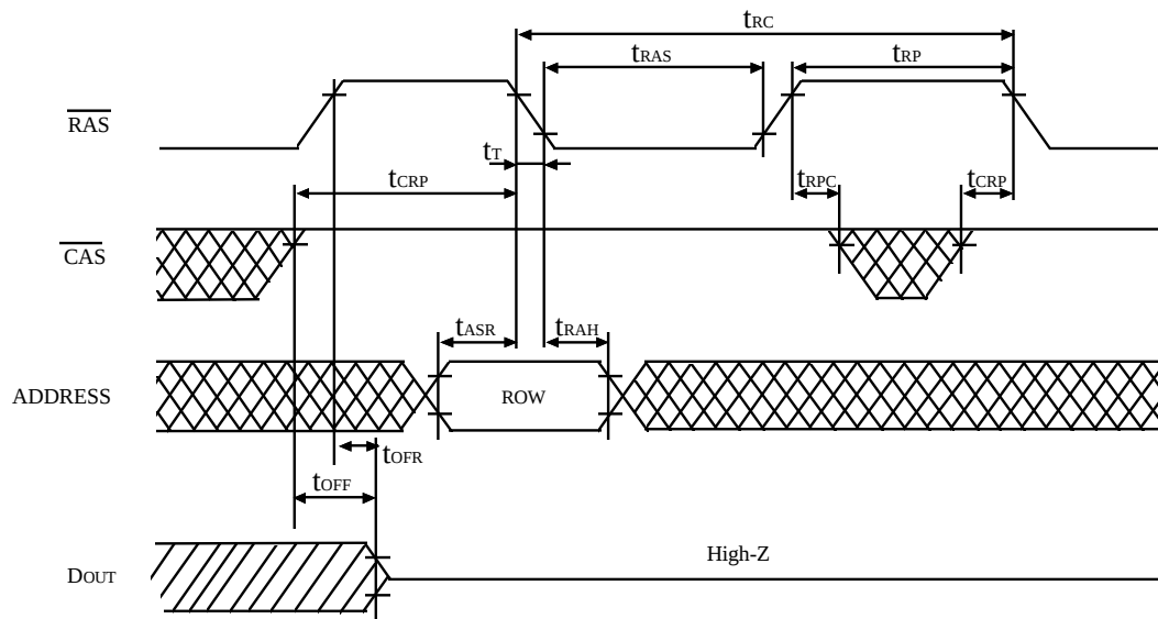
FIGURE 5. \overline{\text{RAS}} ONLY REFRESH CYCLE
