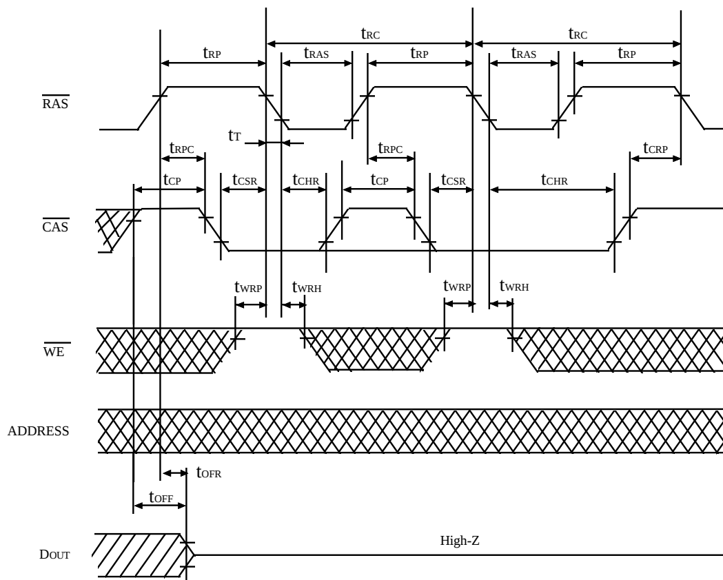
FIGURE 6. \overline{\text{CAS}} BEFORE \overline{\text{RAS}} REFRESH CYCLE
