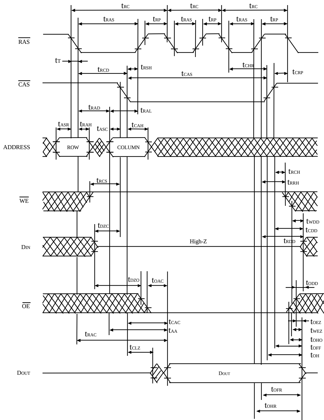
FIGURE 7. HIDDEN REFRESH CYCLE
