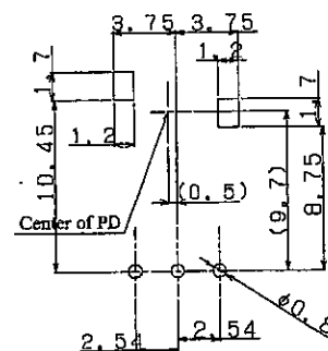
Example of mounting drawing from solder side (Reference)
