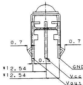
Example of mounting drawing from solder side(Reference)
