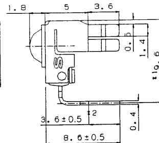
Example of mounting drawing from solder side(Reference)
