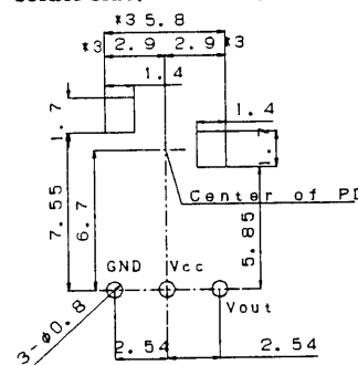
Example of mounting drawing from solder side(Reference)
