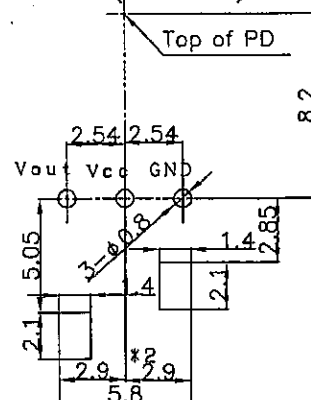
Example of mounting drawing from solder side(Reference)
