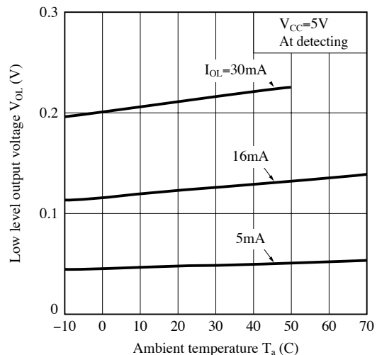
Fig.6 Low Level Output Voltage vs. Ambient Temperature
