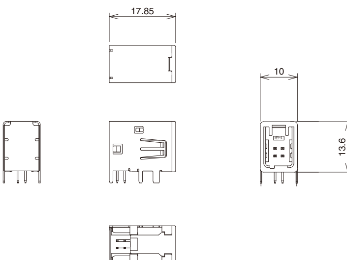
GT17HN-4DP-2DS(A)(10)
