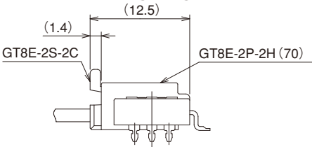
◆Fitting diagram
