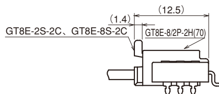
◆Fitting diagram
