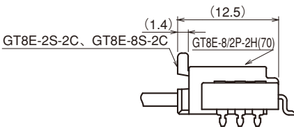
Fitting diagram
